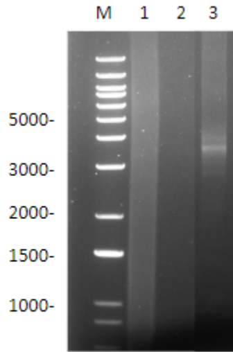
Lane M: DNA 1 KB Ladder Lane 1&2: Samples are not relevant to this batch. Lane 3: Lot 24-028 Purified AAV4-CAG-TdTomato
